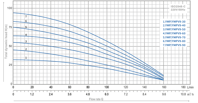
YMP/YMPV9 PERFORMANCE CHART
